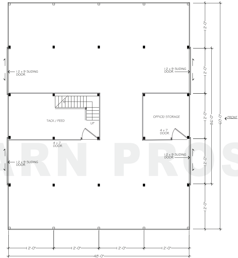
FLOORPLAN - LOWER
