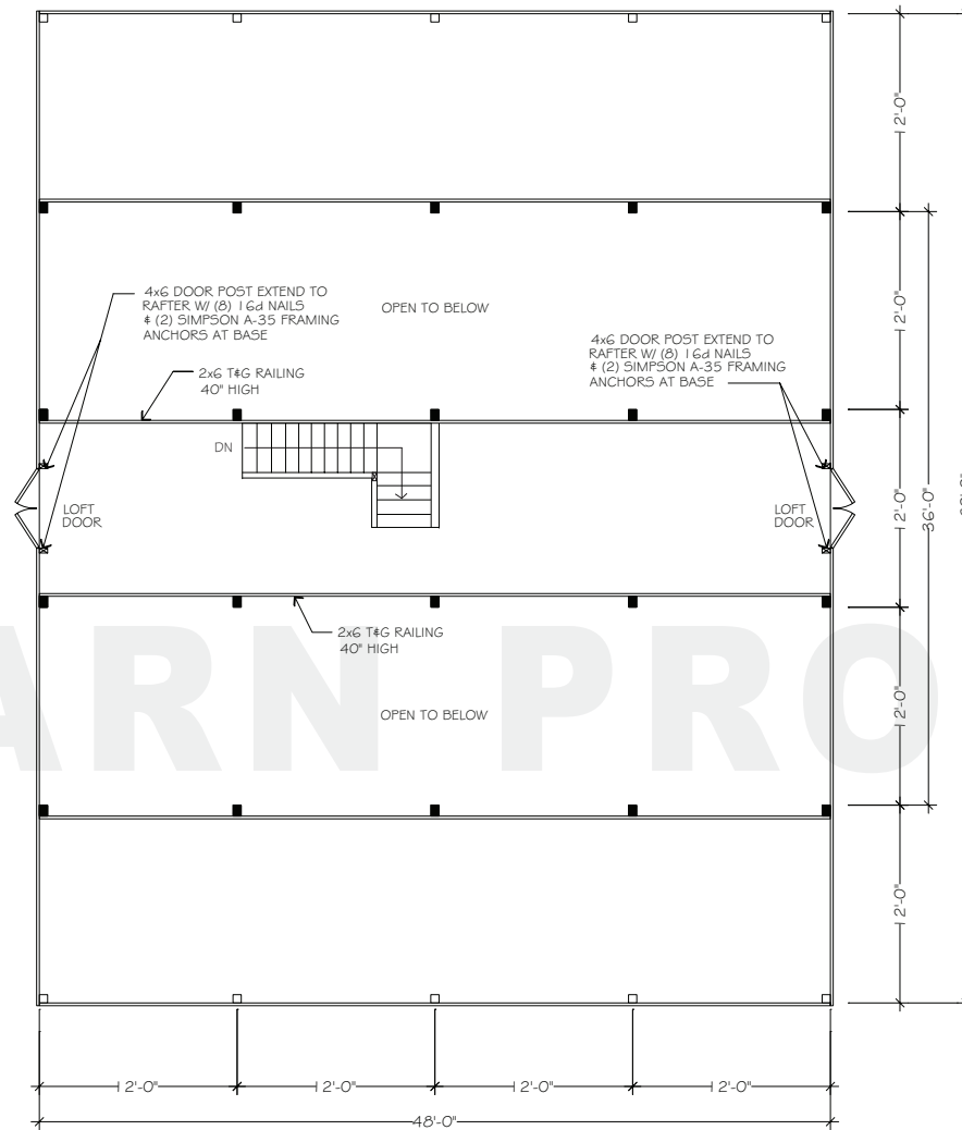
FLOORPLAN - UPPER
