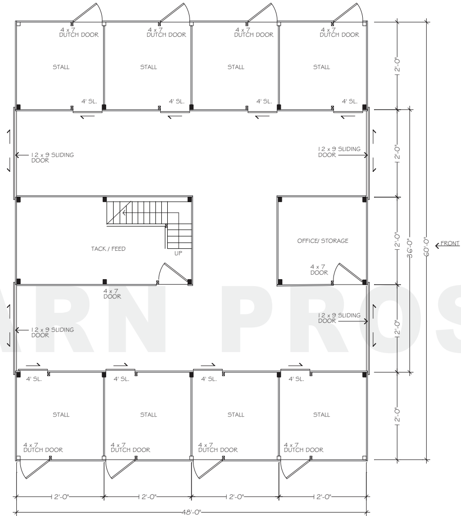
FLOORPLAN - LOWER
