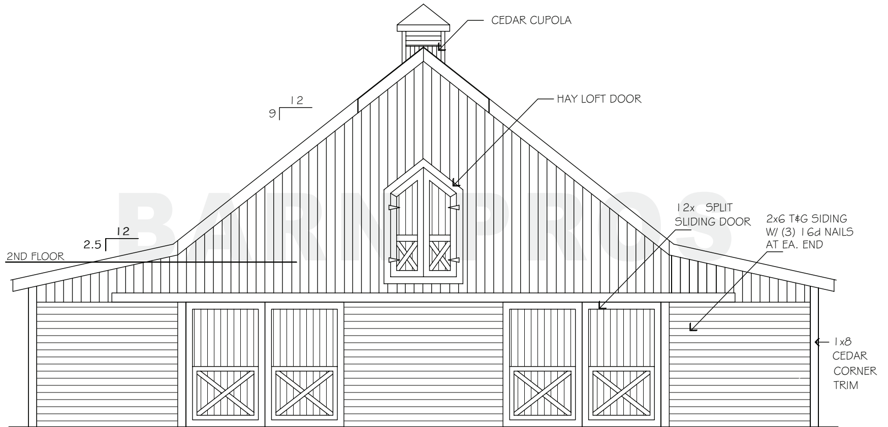
FRONT ELEVATION
