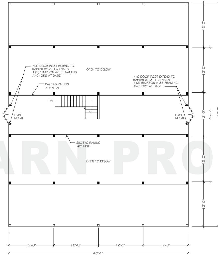
FLOORPLAN - UPPER
