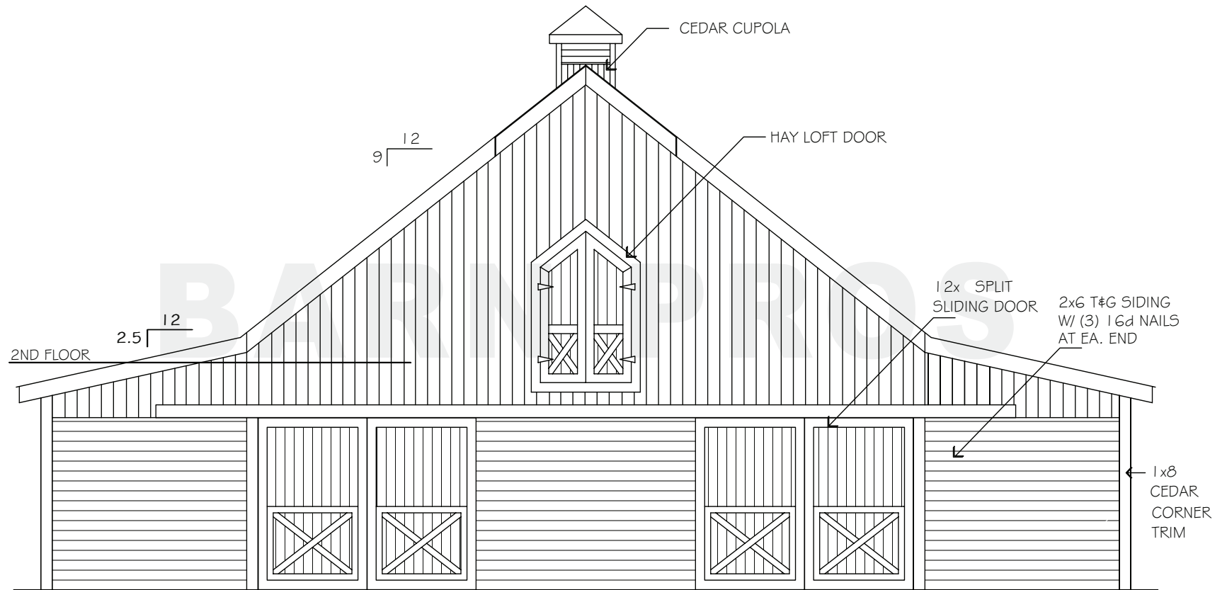
FRONT ELEVATION
