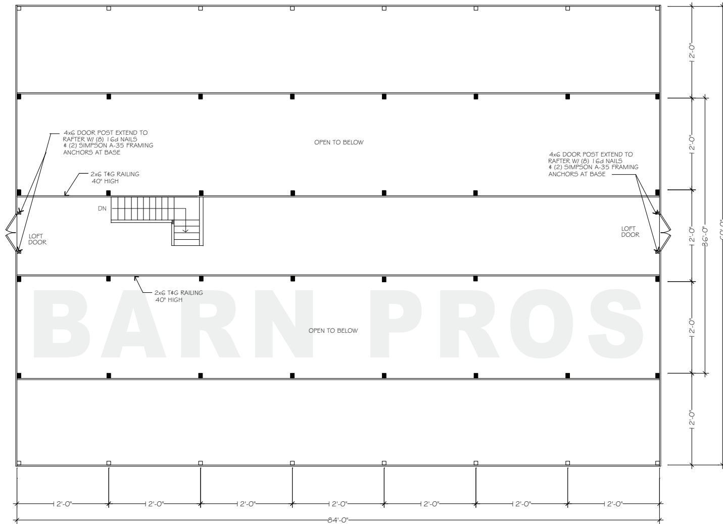
FLOORPLAN - UPPER
