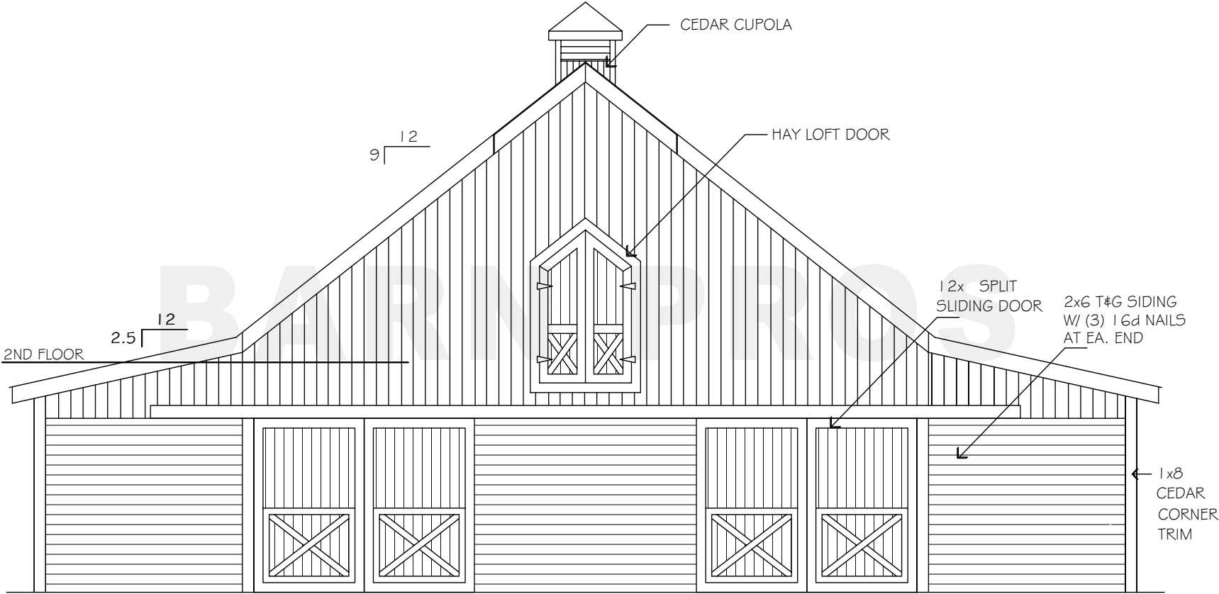
FRONT ELEVATION
