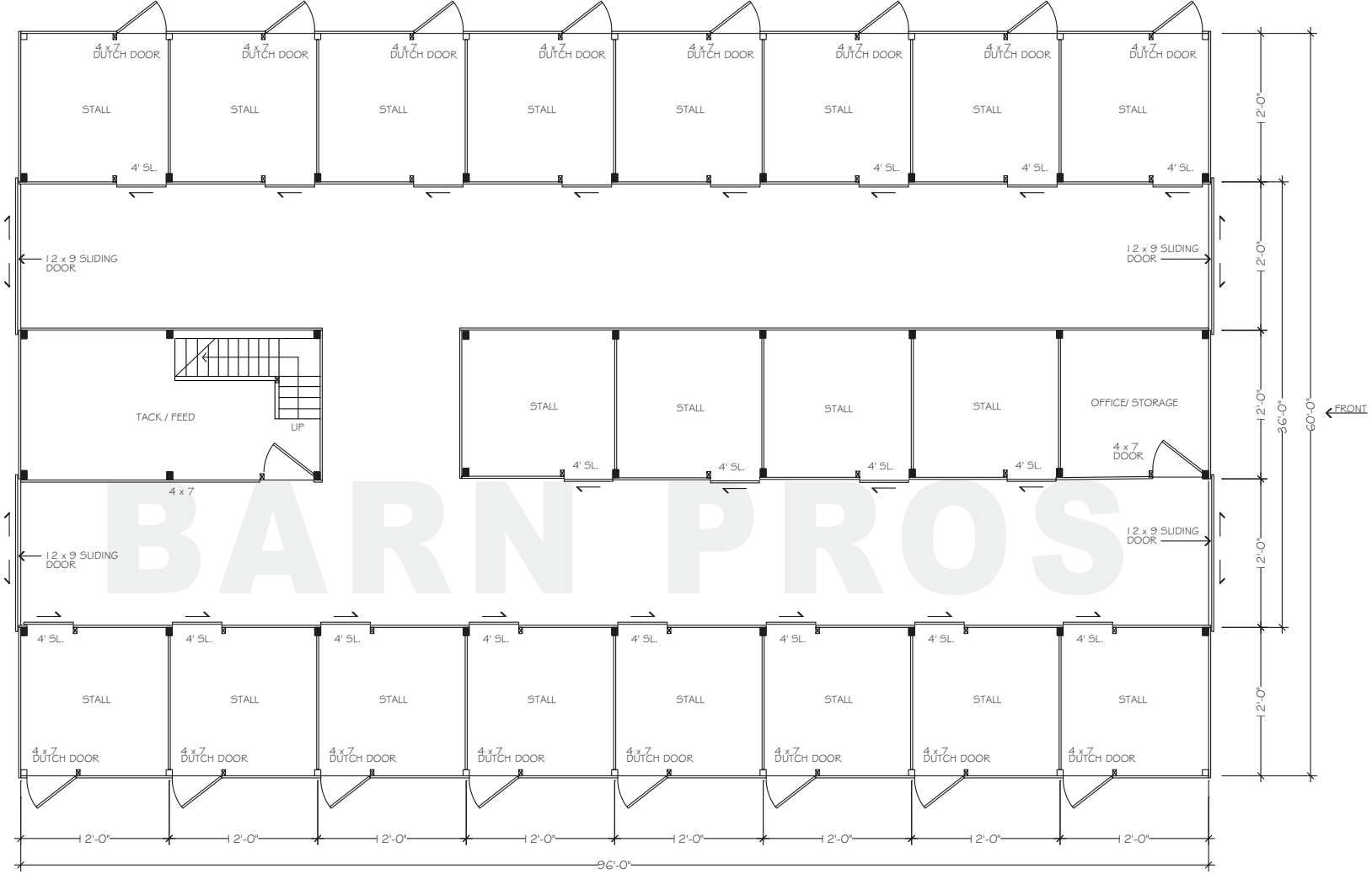
FLOORPLAN - LOWER
