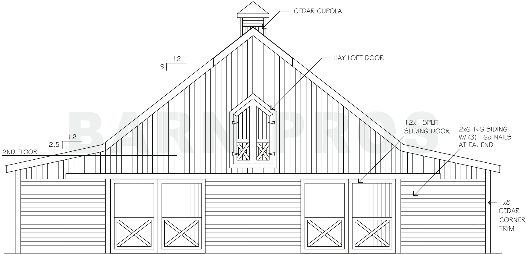
REAR ELEVATION
