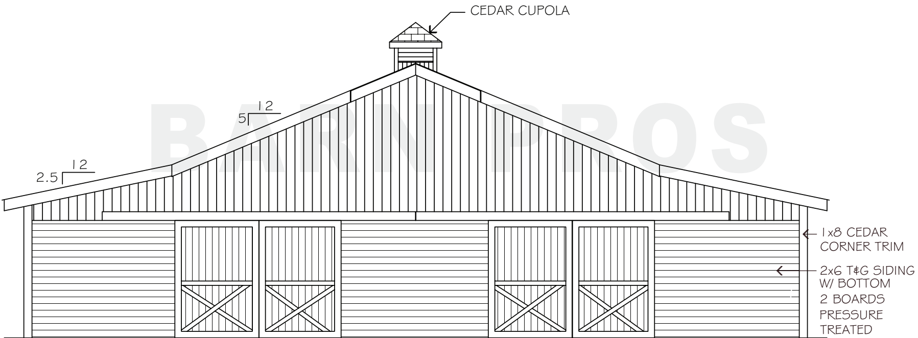
FRONT ELEVATION
