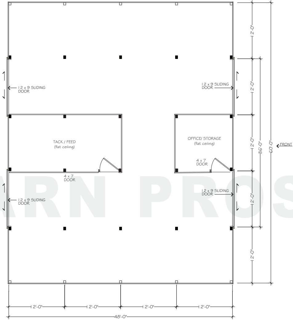
FLOORPLAN - LOWER
