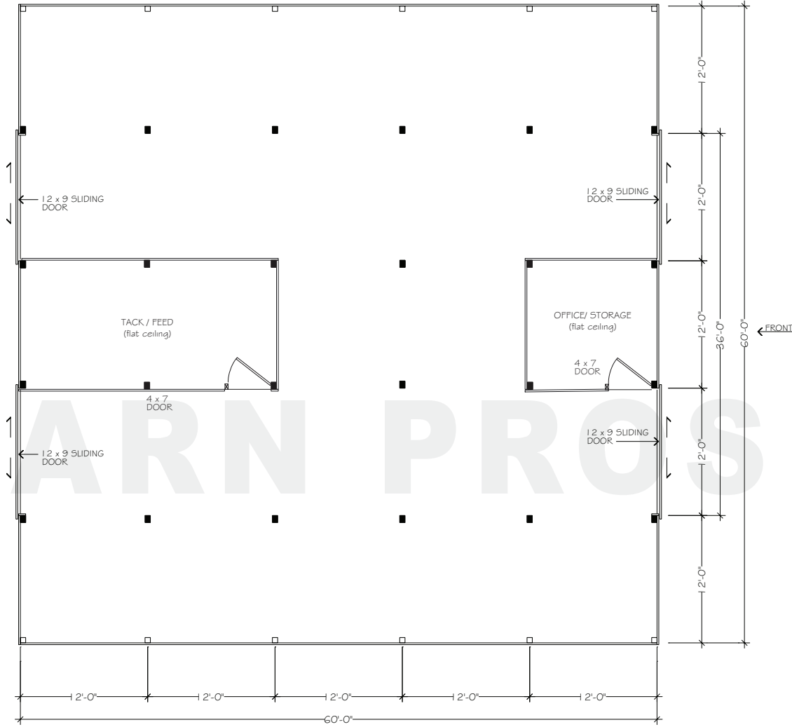
FLOORPLAN - LOWER
