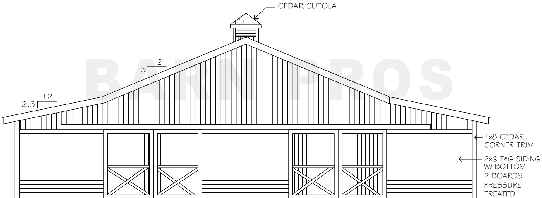
REAR ELEVATION
