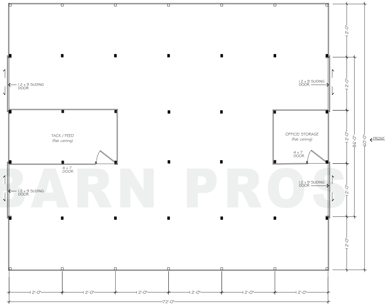
FLOORPLAN - LOWER
