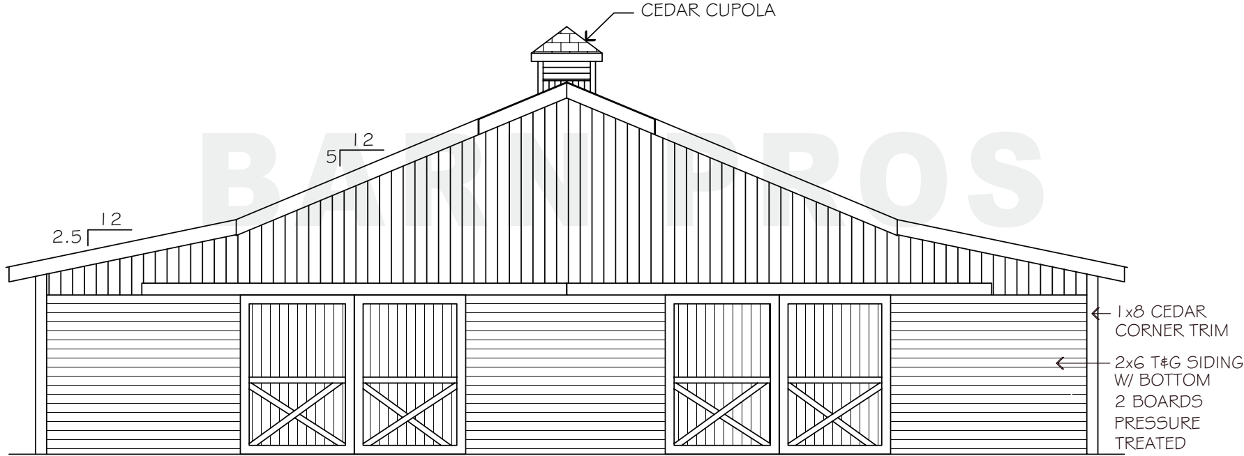
FRONT ELEVATION
