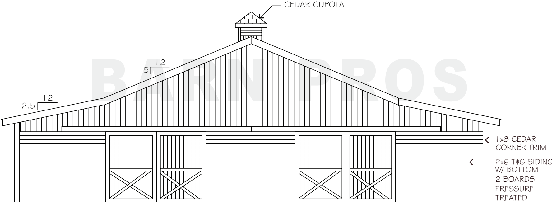
REAR ELEVATION
