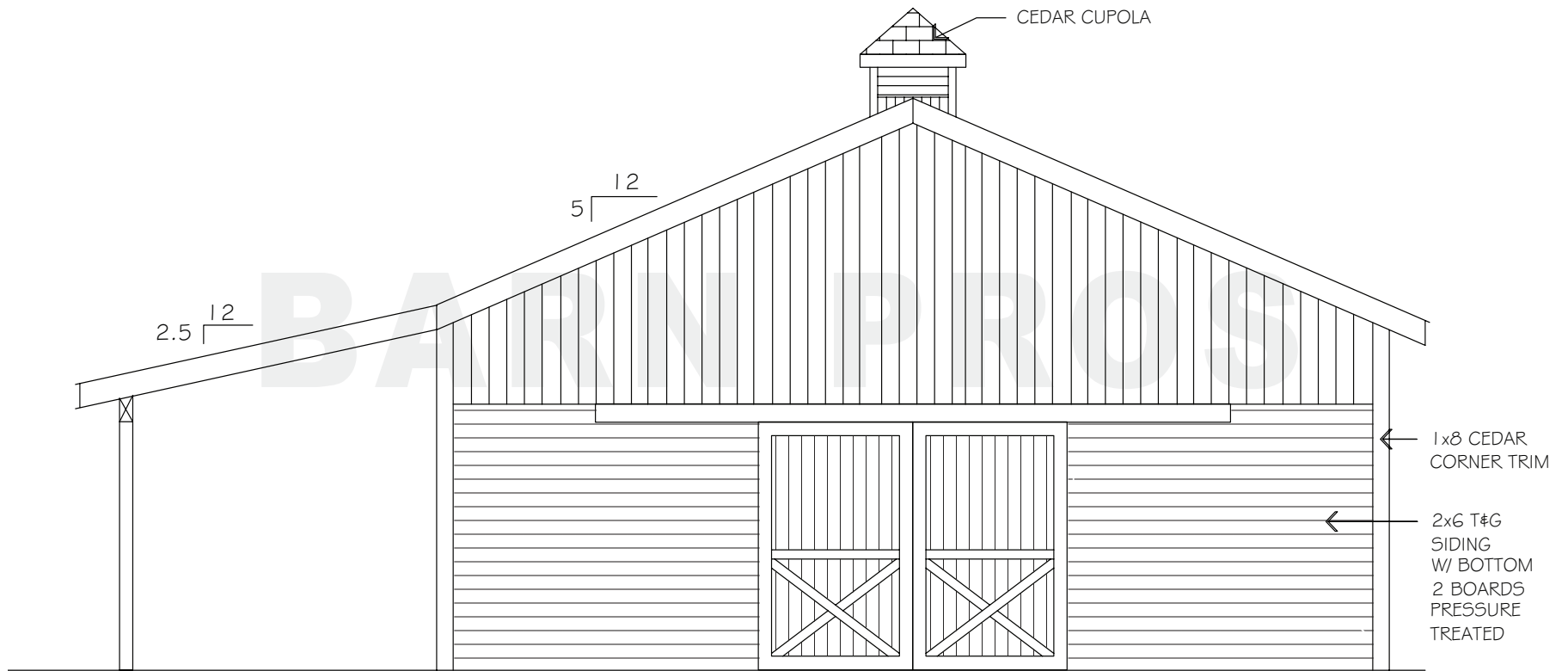
REAR ELEVATION
