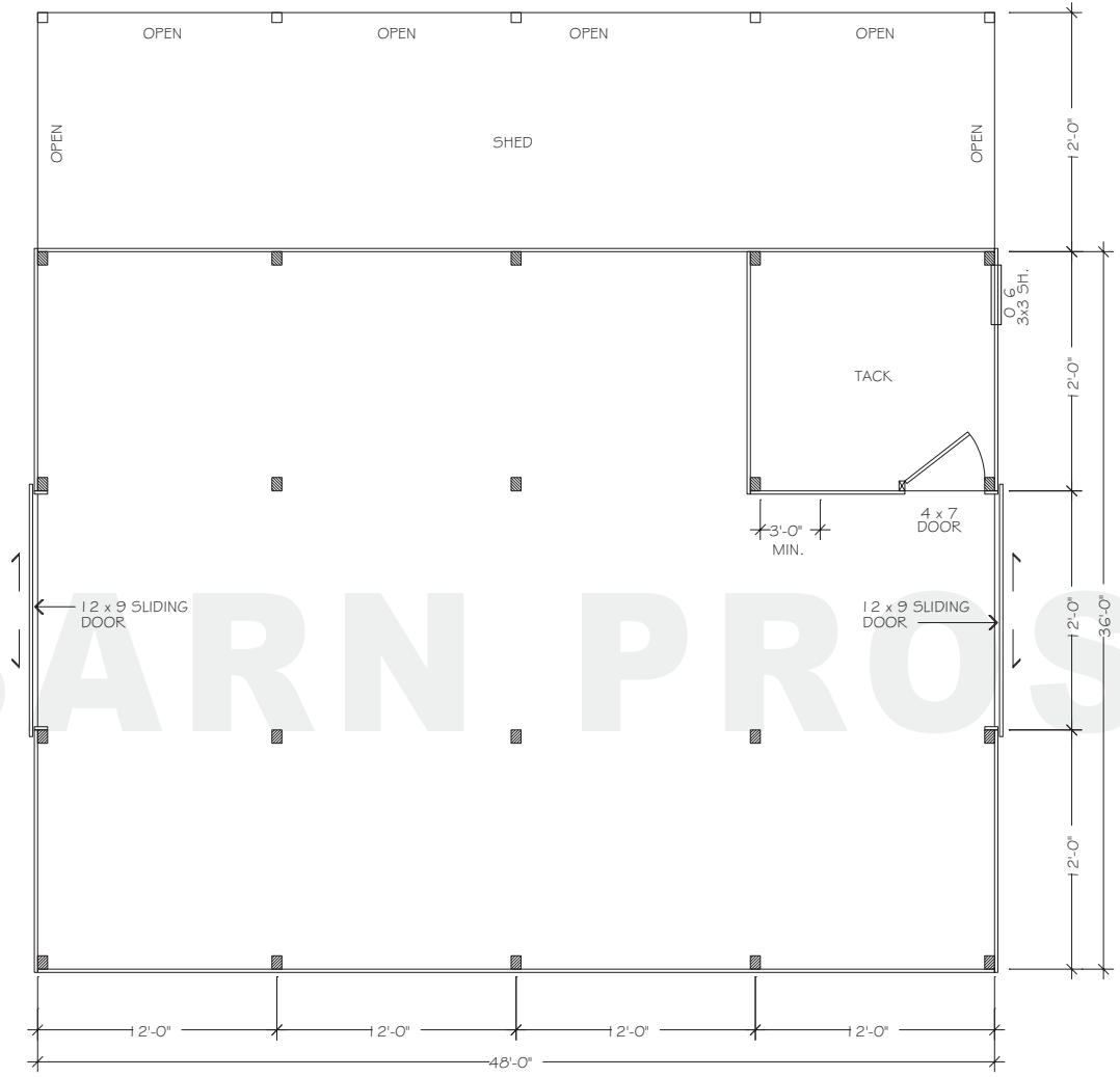
FLOORPLAN - LOWER
