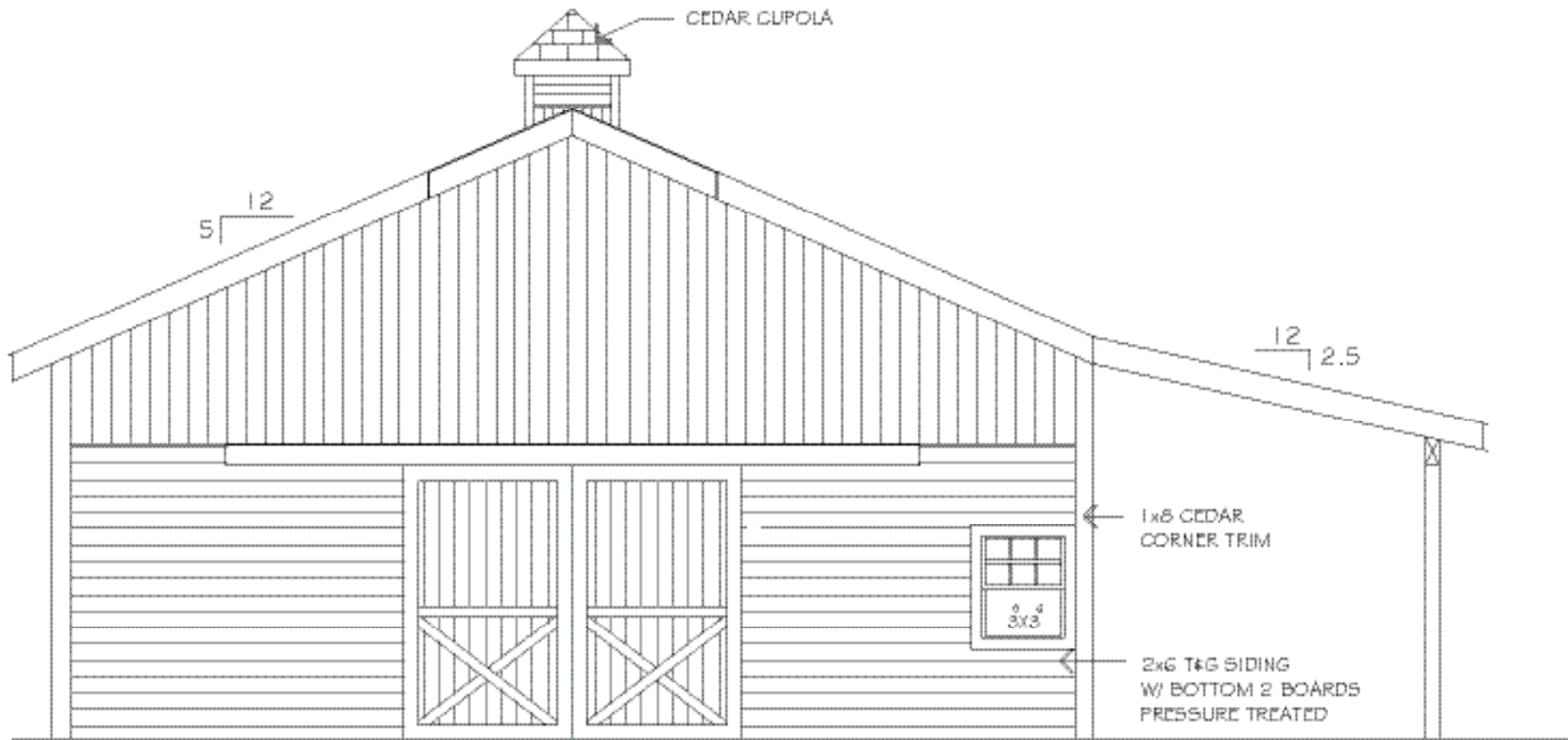
FRONT ELEVATION
