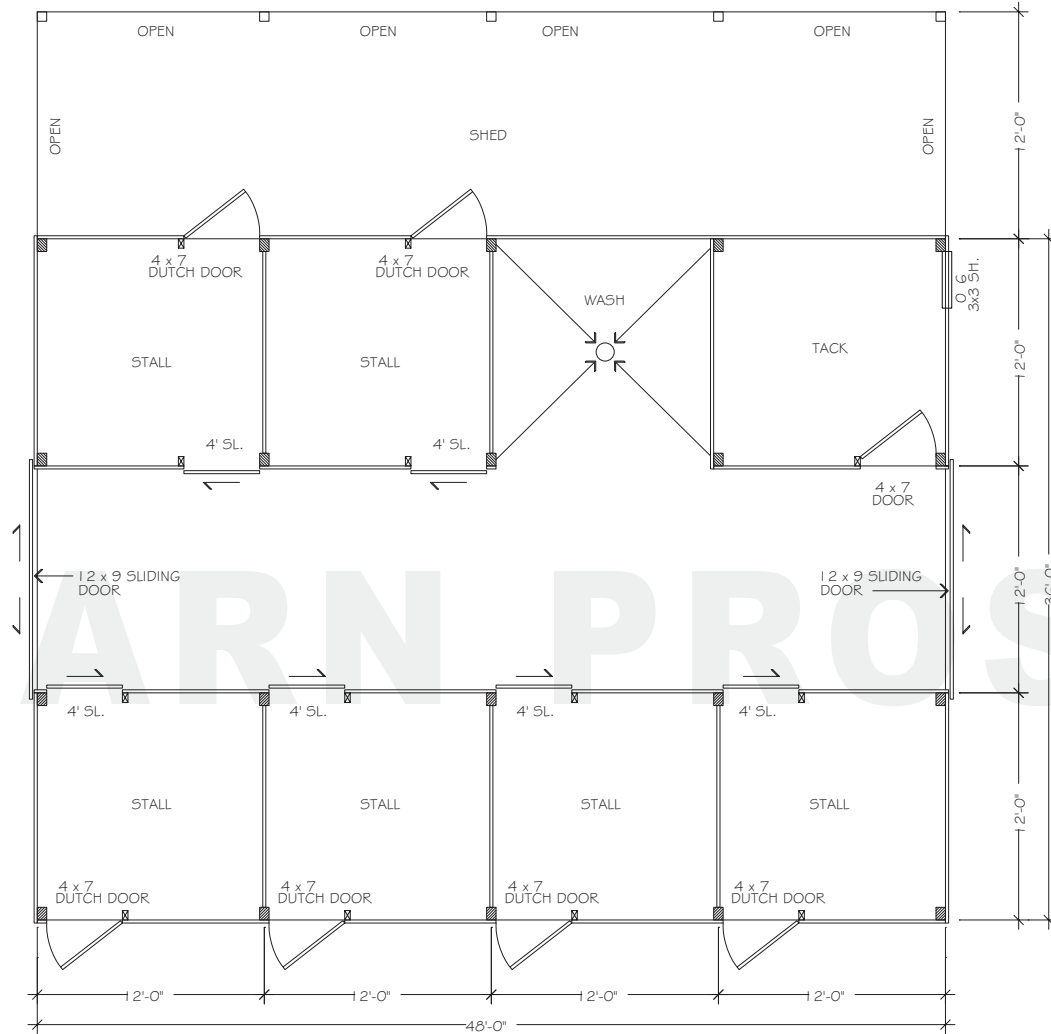
FLOORPLAN - LOWER
