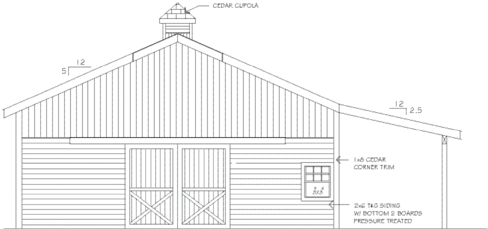
FRONT ELEVATION
