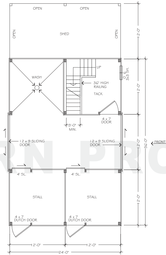
FLOORPLAN - LOWER
