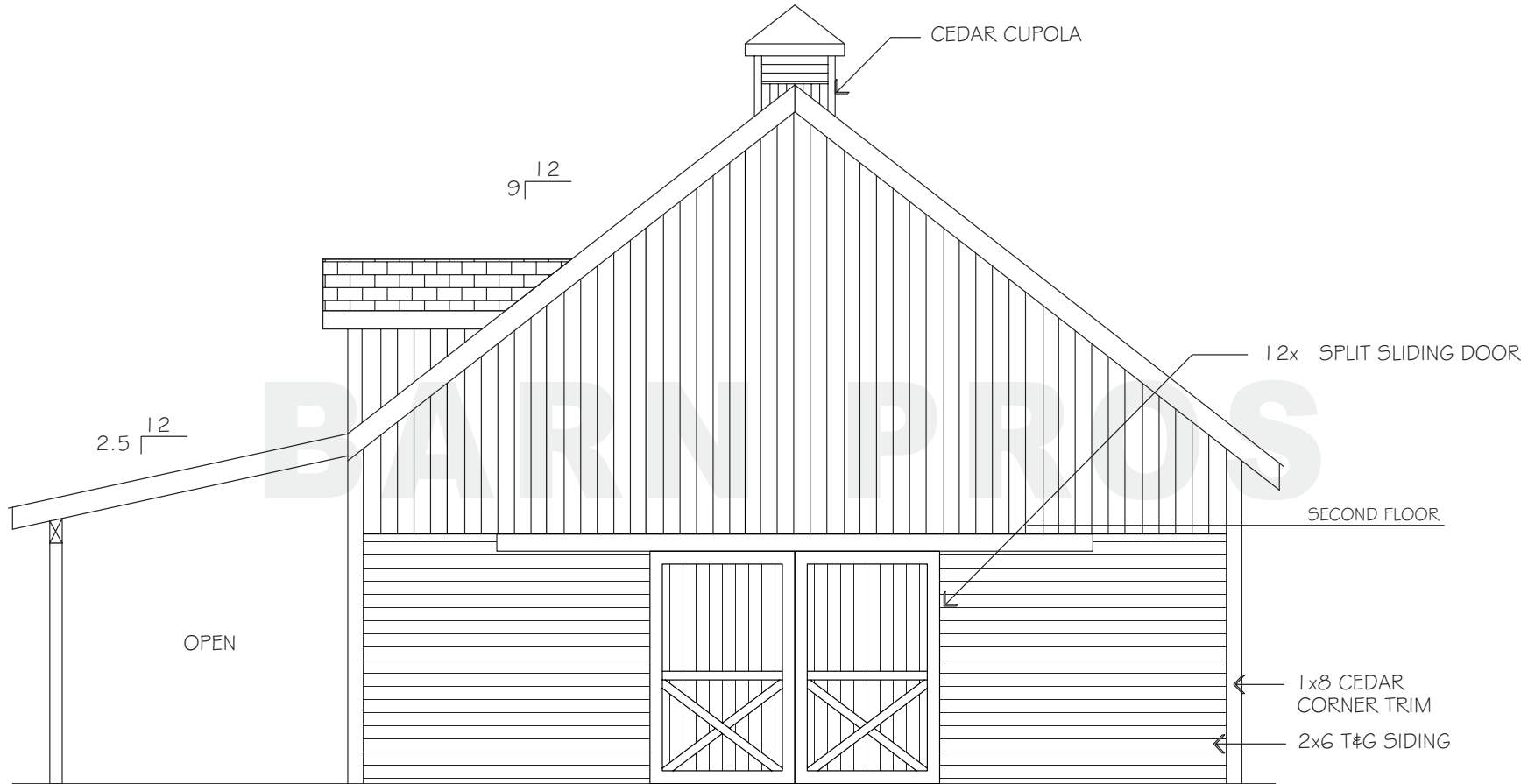
REAR ELEVATION
