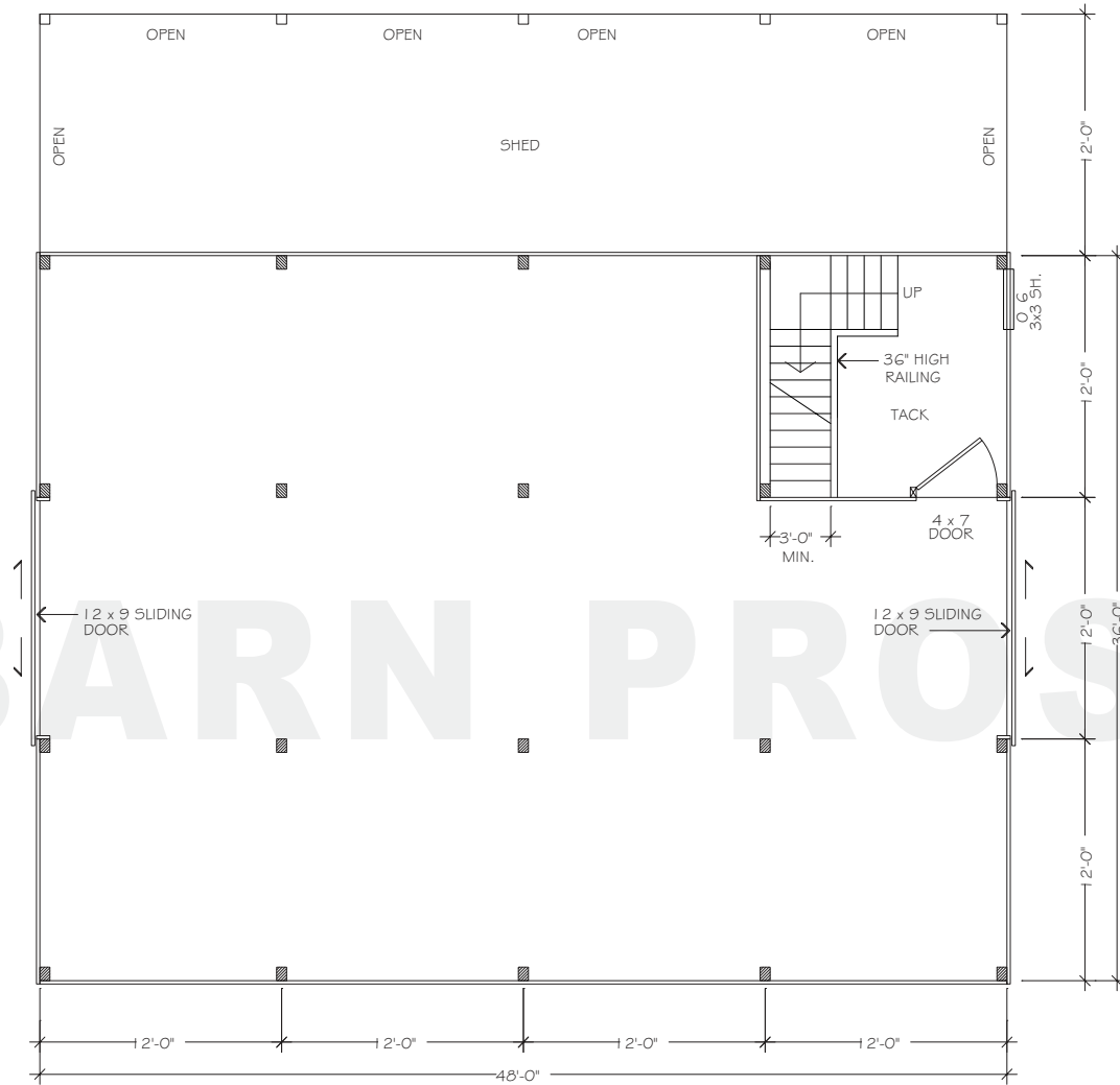
FLOORPLAN - LOWER
