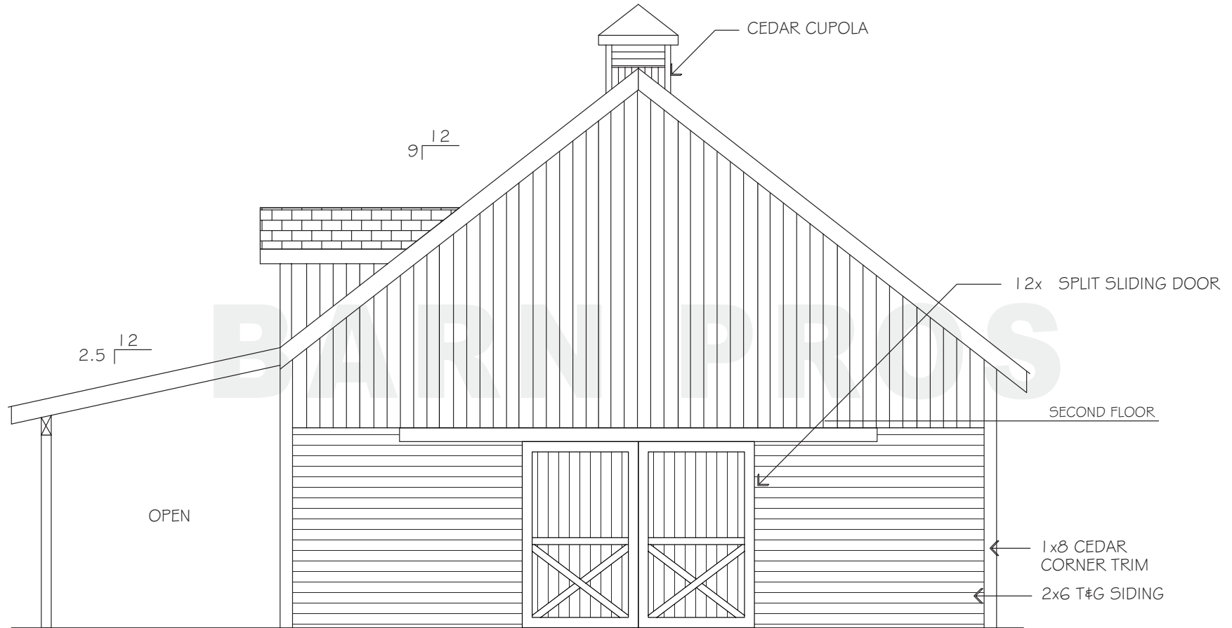
REAR ELEVATION
