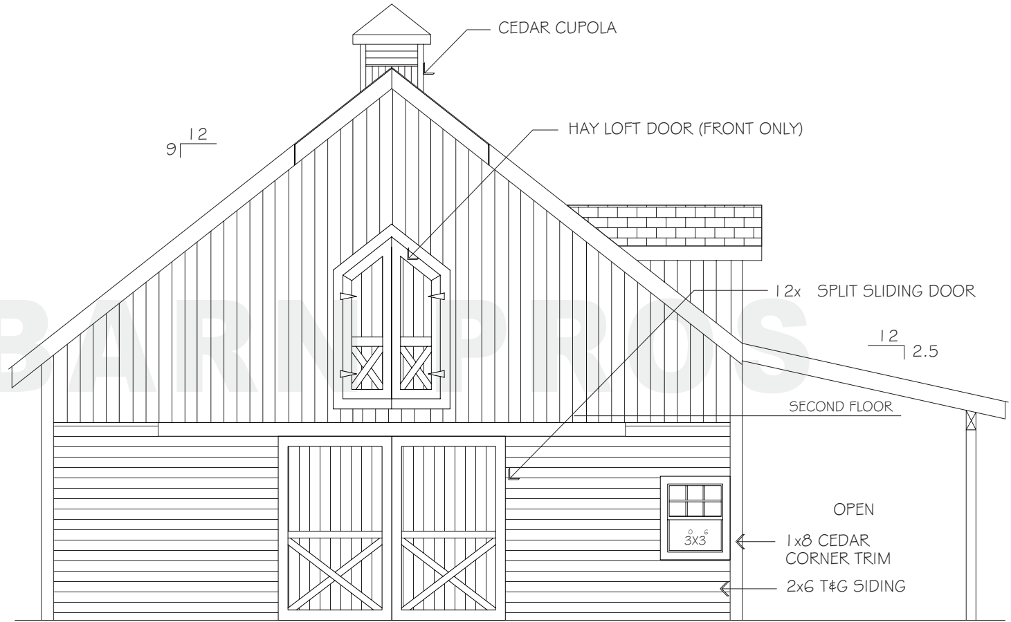
FRONT ELEVATION
