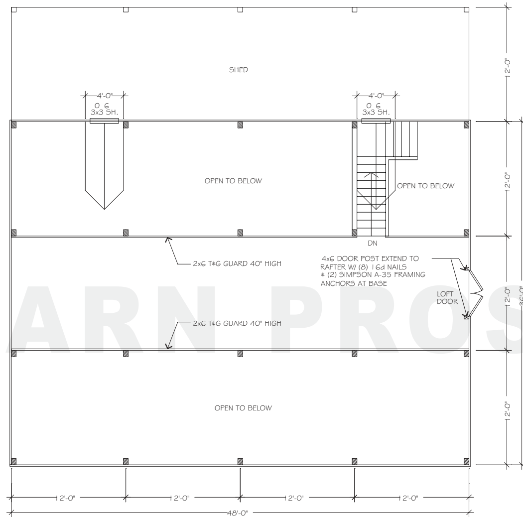
FLOORPLAN - UPPER
