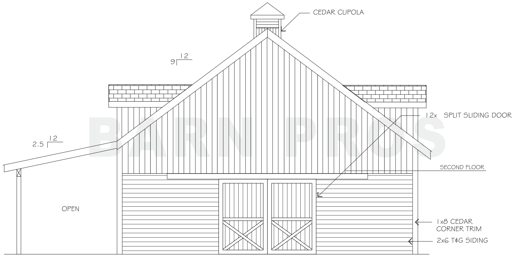
REAR ELEVATION
