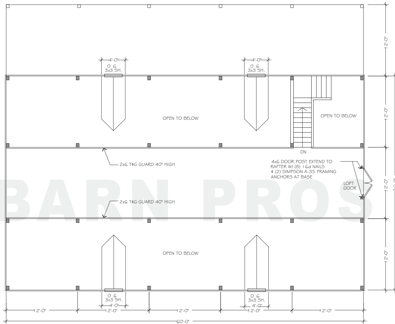
FLOORPLAN - UPPER
