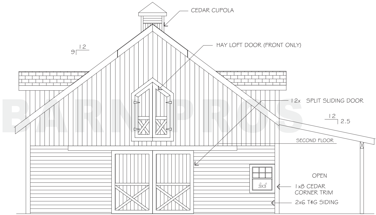
FRONT ELEVATION
