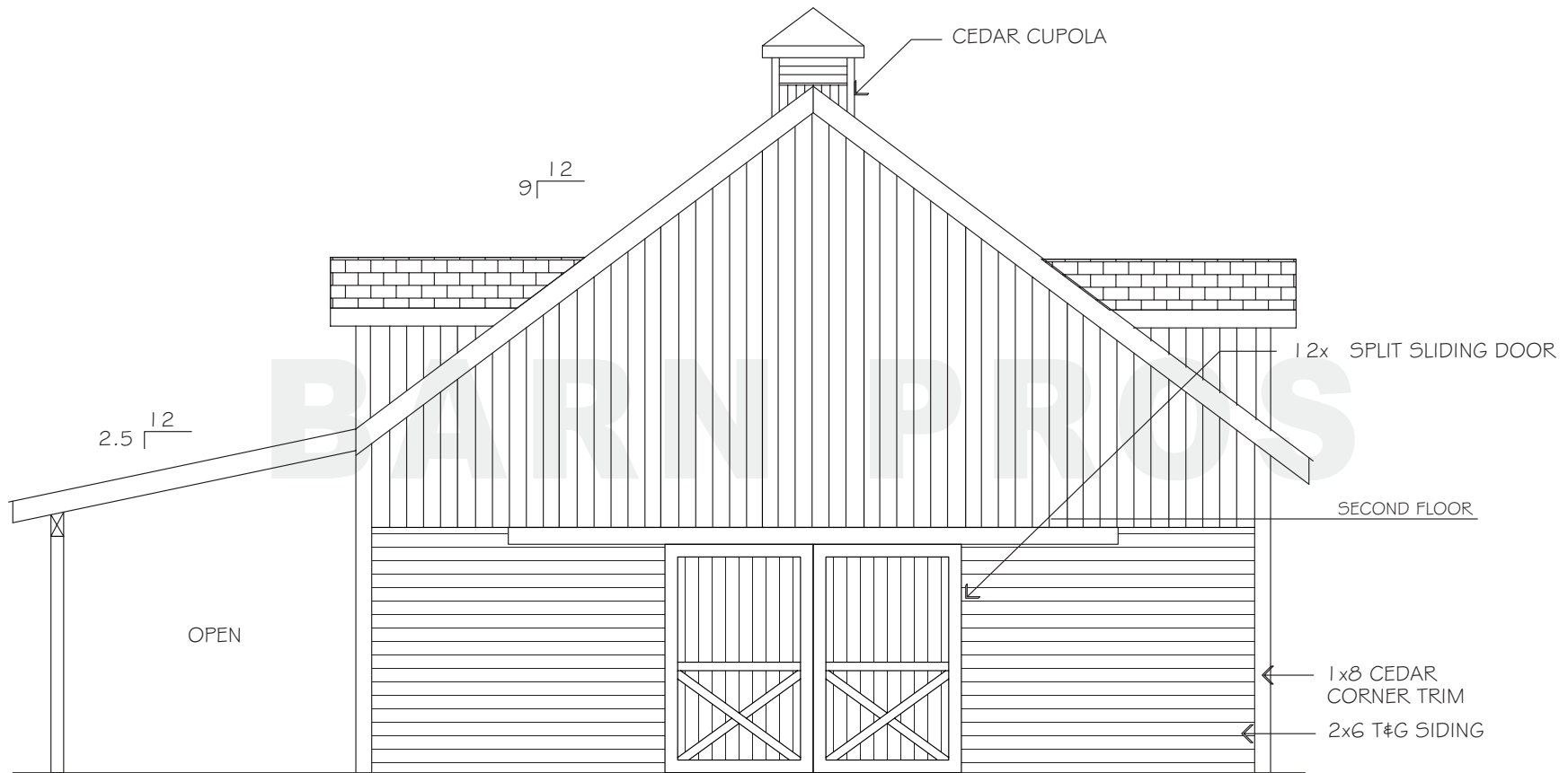
REAR ELEVATION
