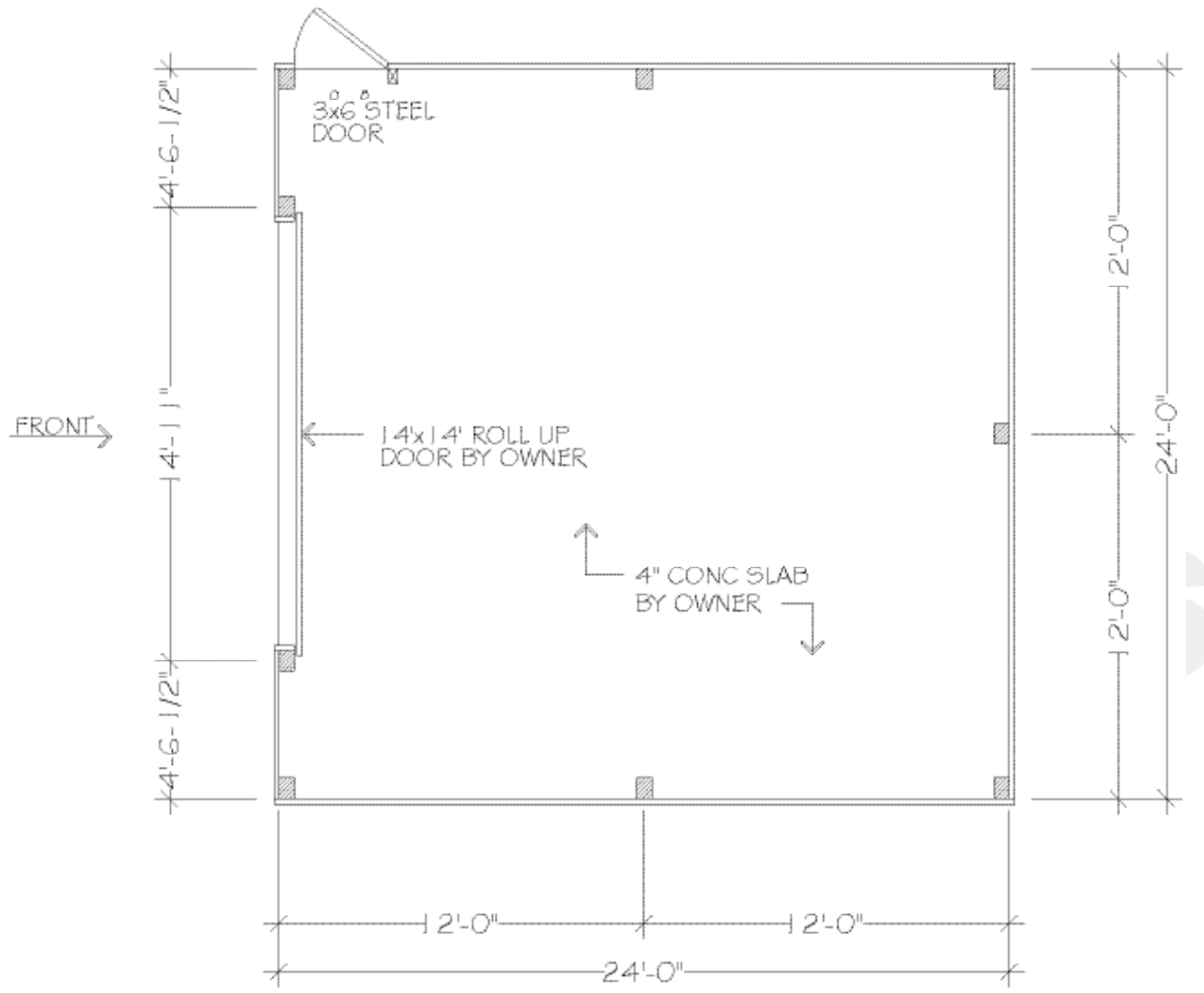
FLOORPLAN - LOWER
