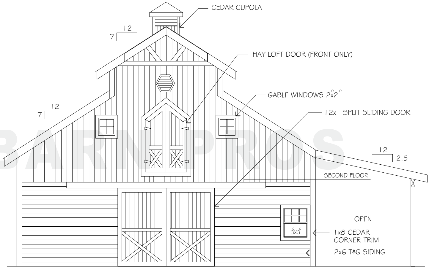
FRONT ELEVATION
