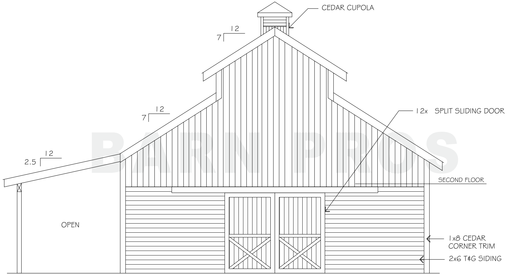
REAR ELEVATION
