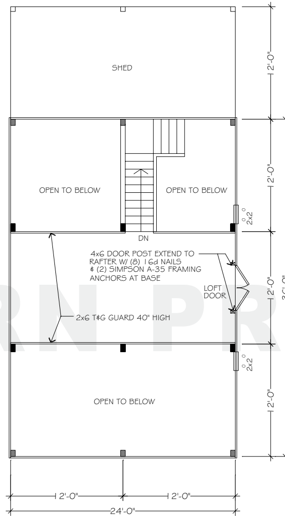
FLOORPLAN - UPPER
