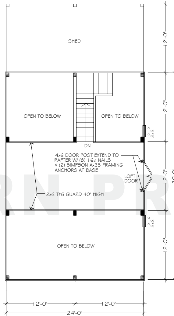
FLOORPLAN - UPPER
