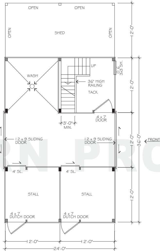
FLOORPLAN - LOWER
