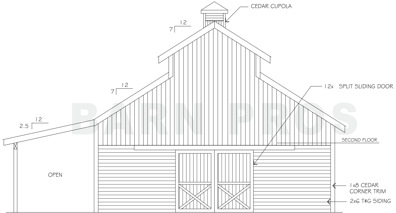
REAR ELEVATION
