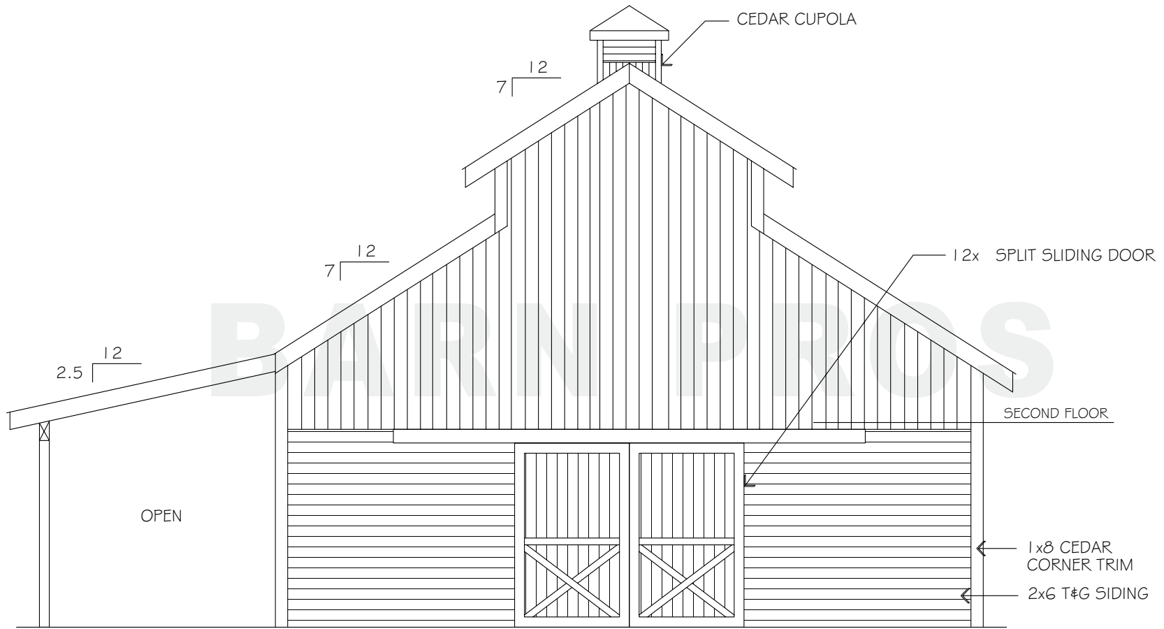
REAR ELEVATION
