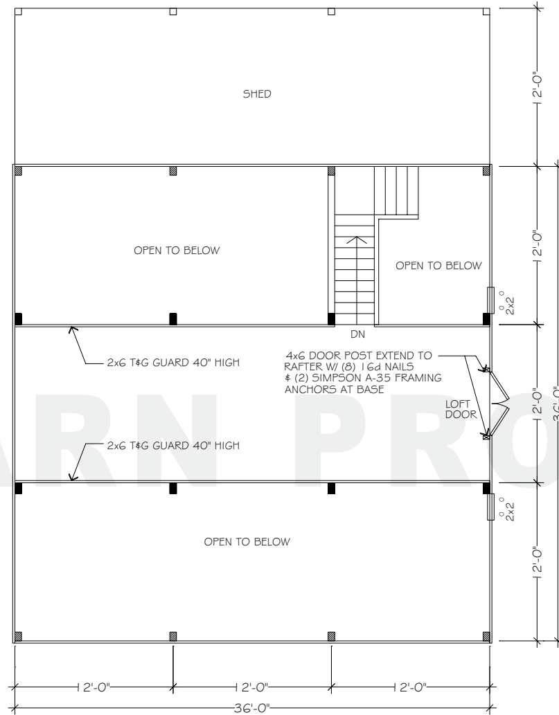
FLOORPLAN - UPPER
