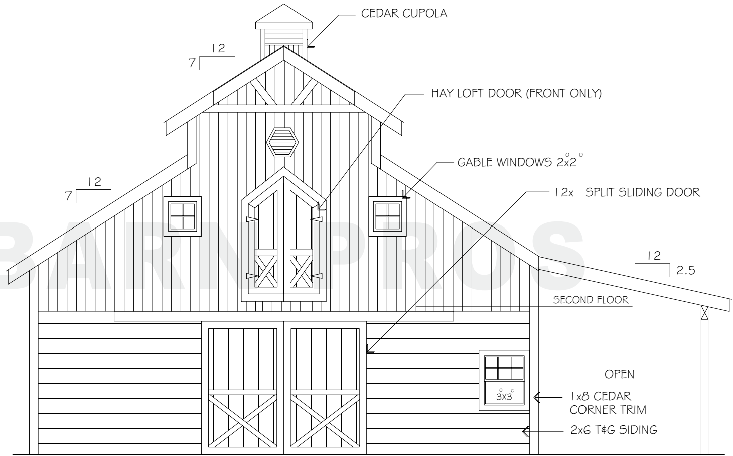
FRONT ELEVATION
