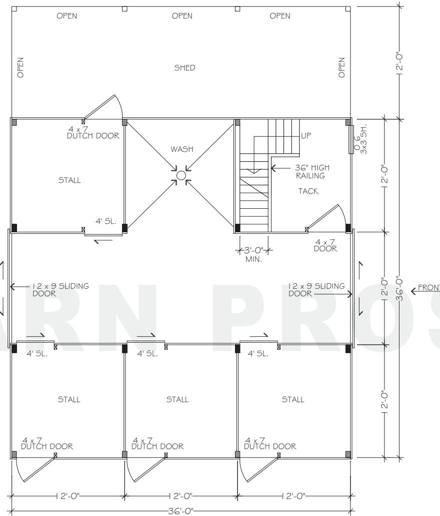
FLOORPLAN - LOWER
