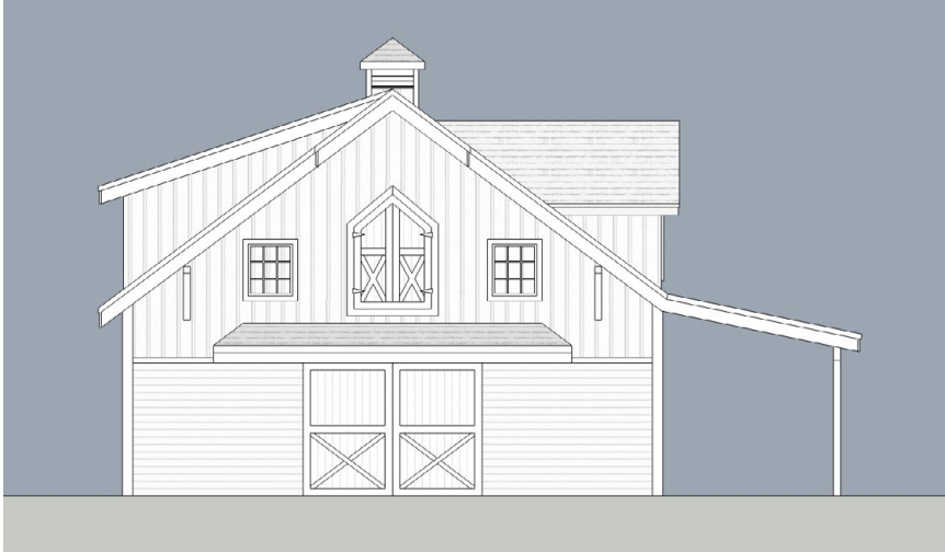
Front Elevation
