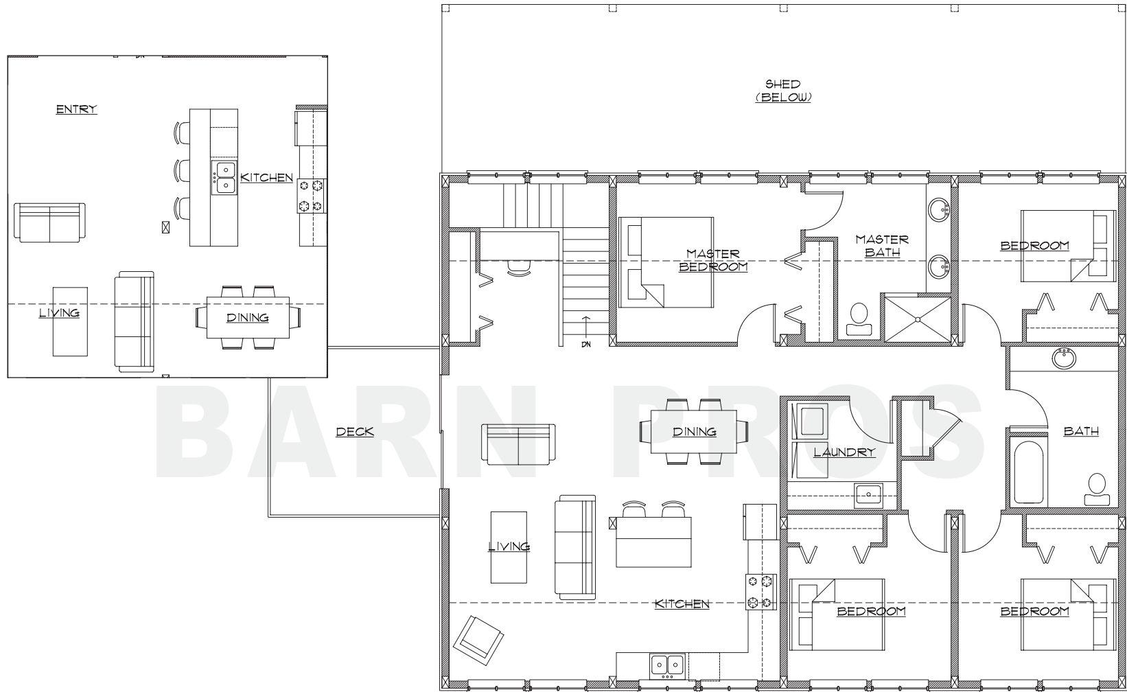
PROPOSED FLOORPLAN - UPPER Model D - Layout 1(right) & Layout 2(inset, upper left)
