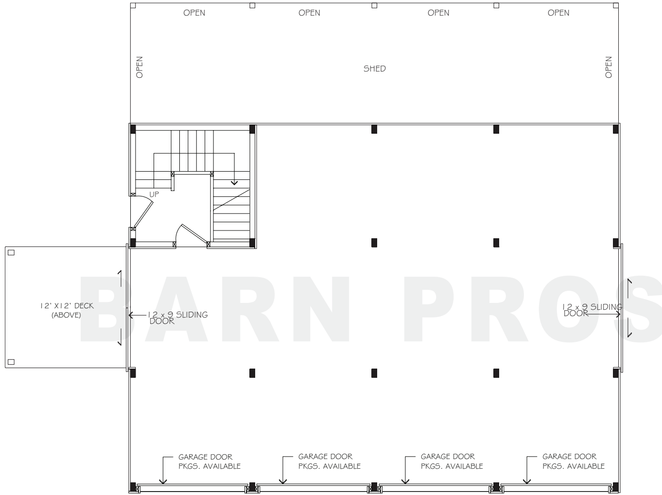
FLOORPLAN - LOWER
