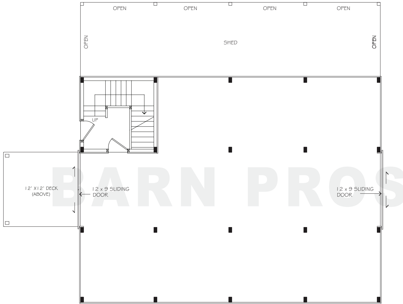
FLOORPLAN - LOWER
