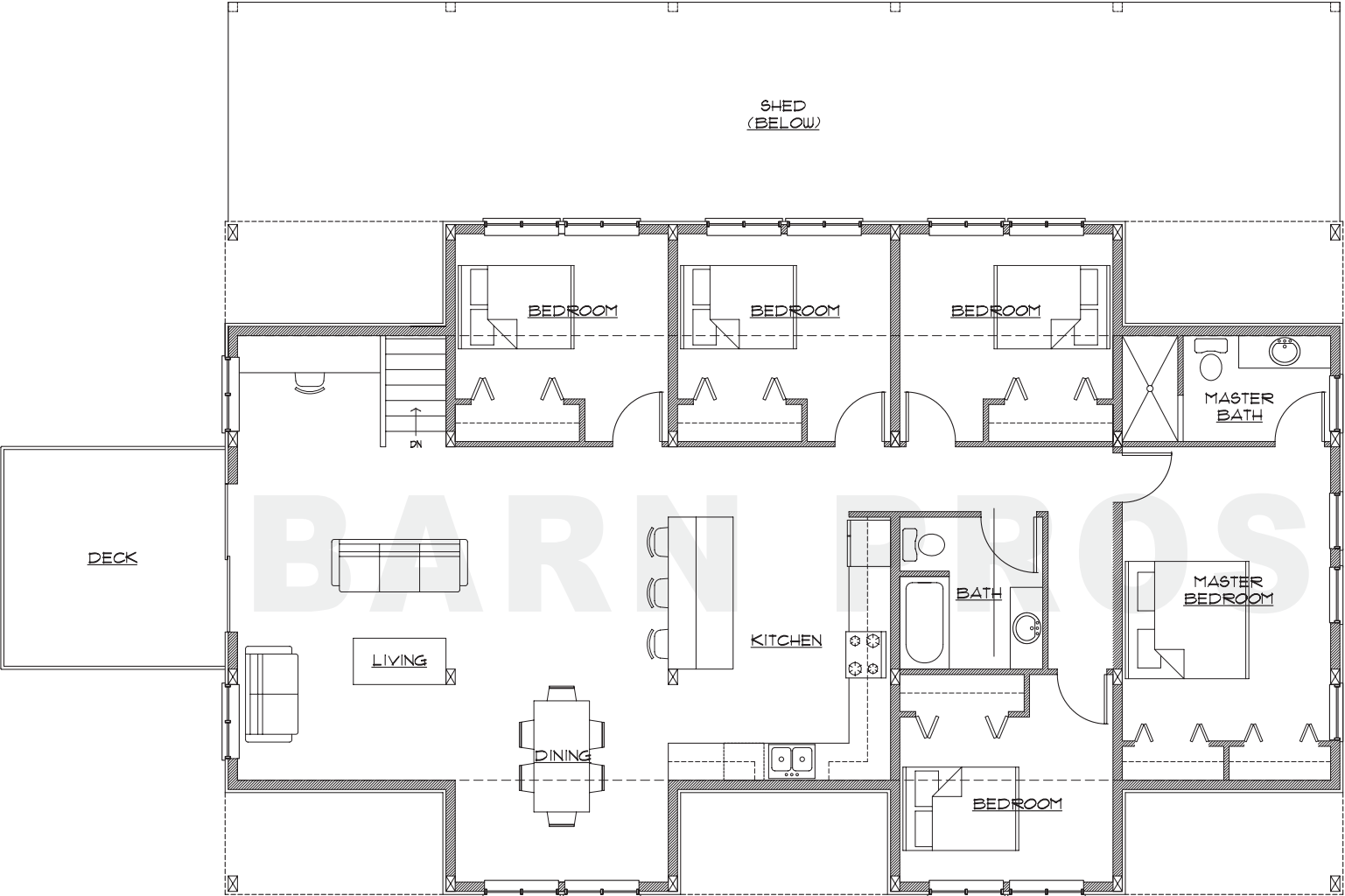
PROPOSED FLOORPLAN - UPPER Model B
