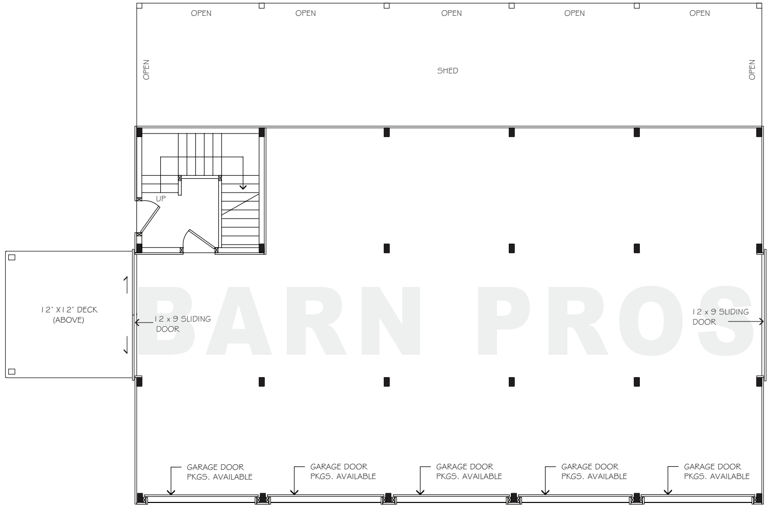
FLOORPLAN - LOWER
