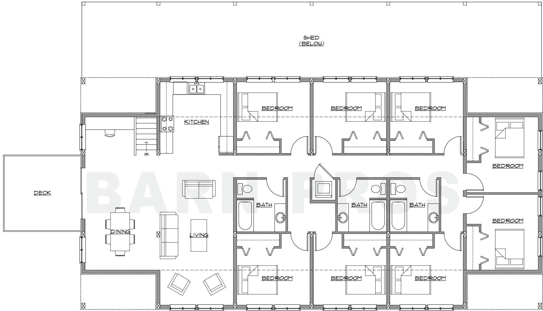
PROPOSED FLOORPLAN - UPPER Model D
