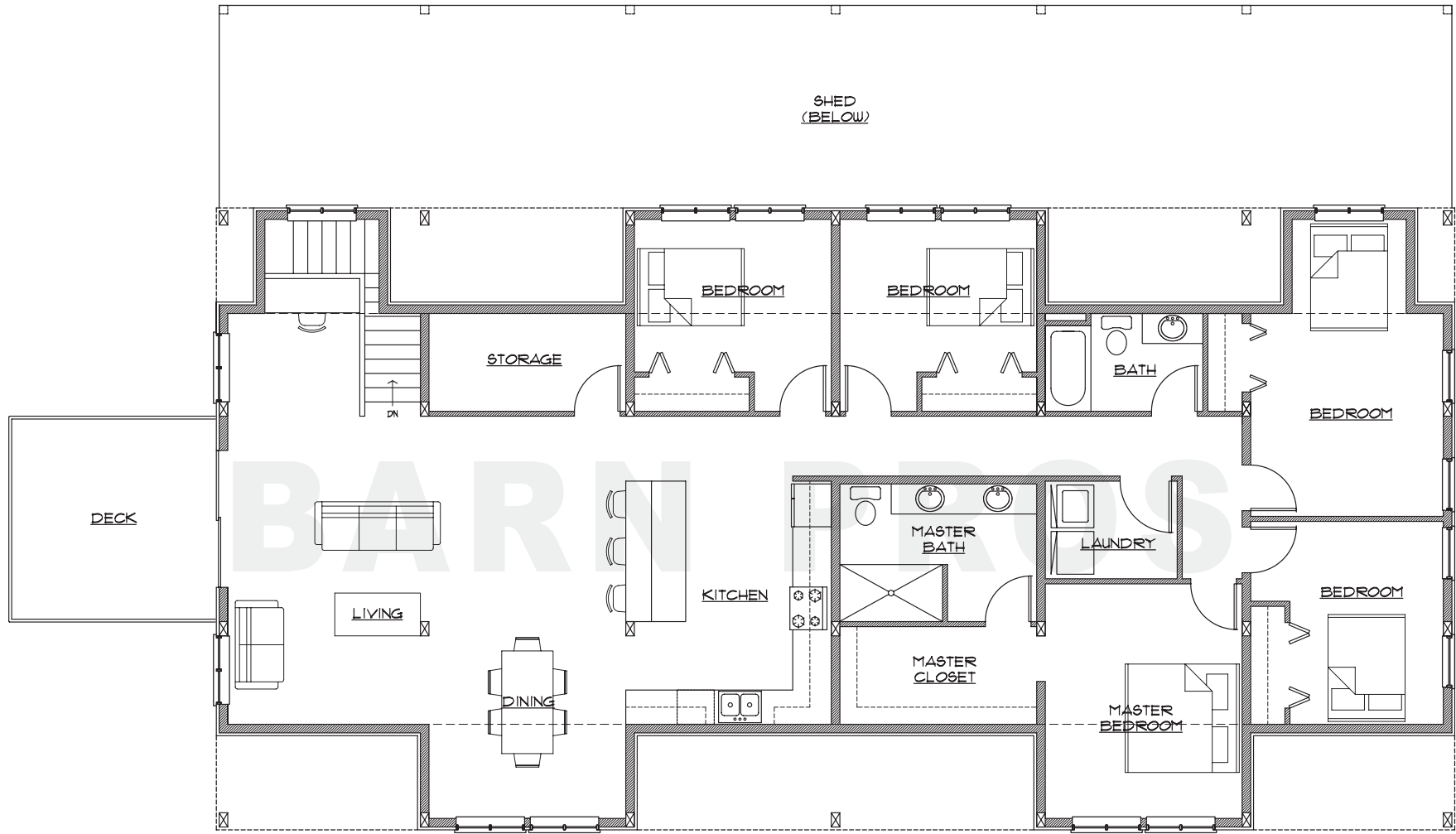
PROPOSED FLOORPLAN - UPPER Model B
