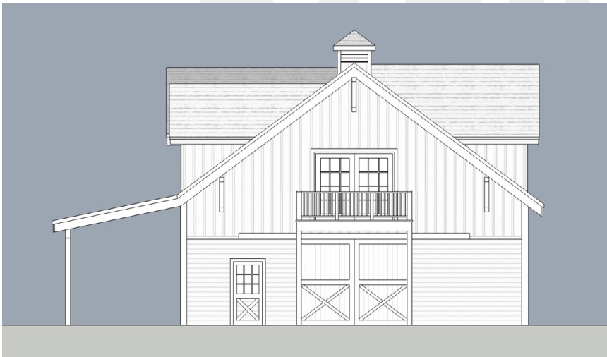
Rear Elevation
