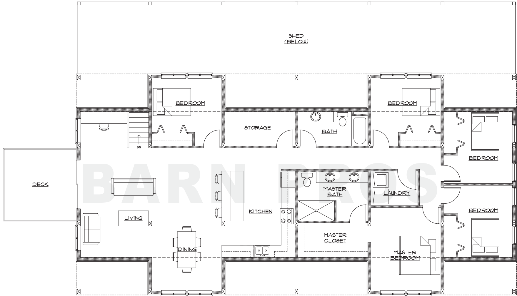
PROPOSED FLOORPLAN - UPPER Model A
