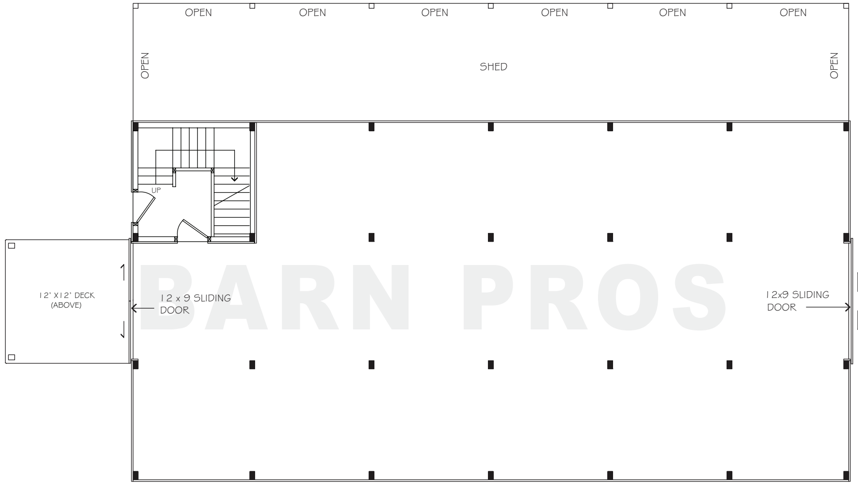
FLOORPLAN - LOWER
