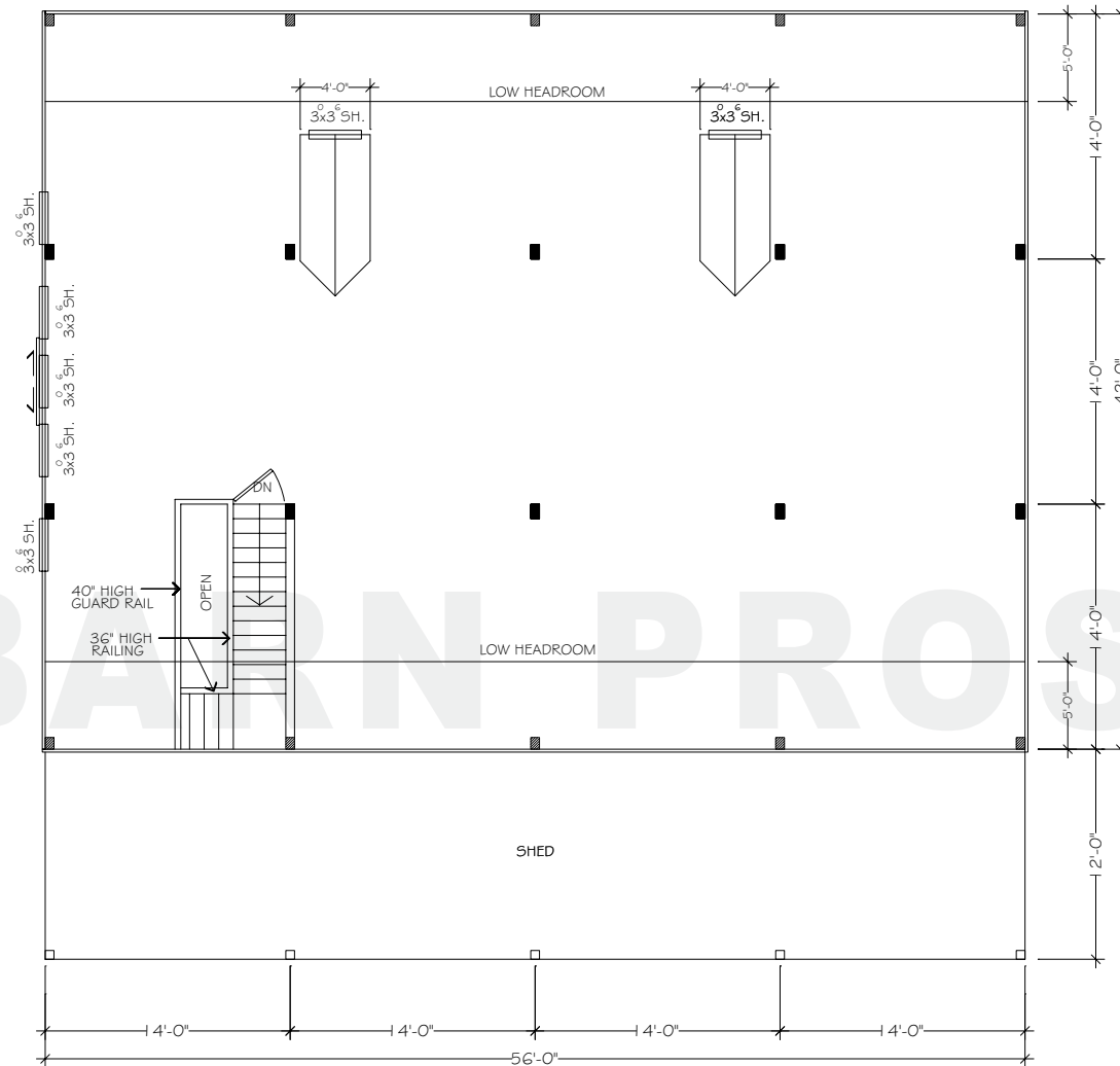
FLOORPLAN - UPPER
