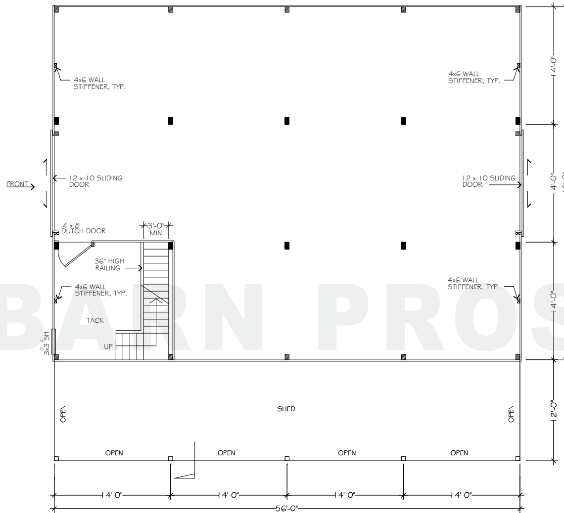
FLOORPLAN - LOWER
