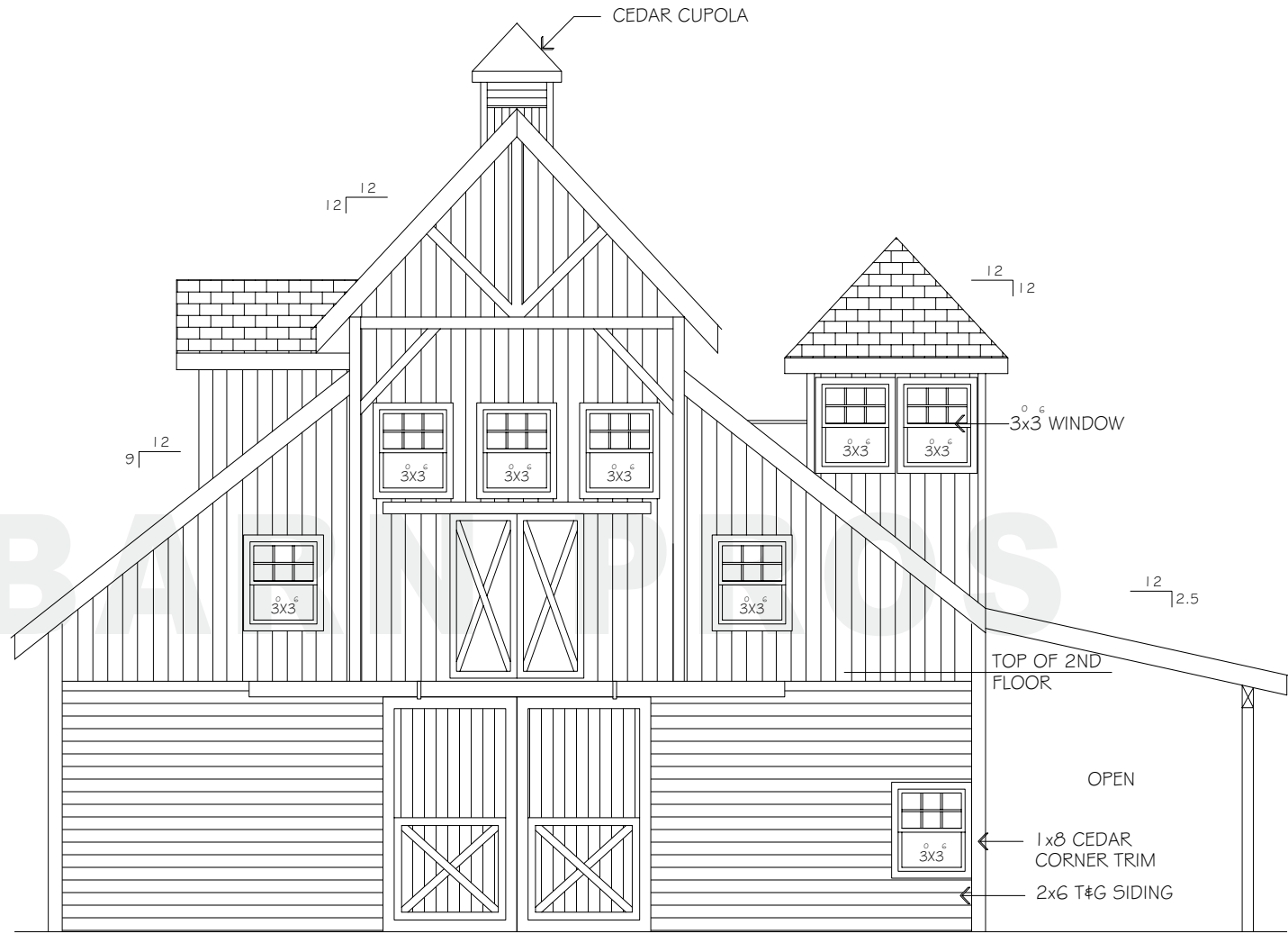
FRONT ELEVATION
