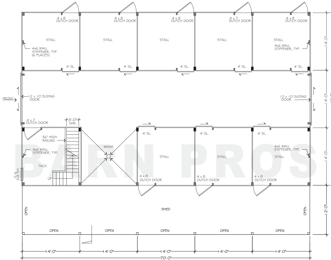
FLOORPLAN - LOWER
