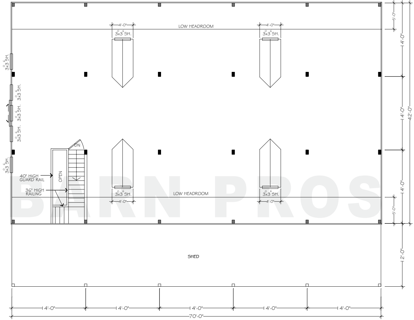
FLOORPLAN - UPPER
