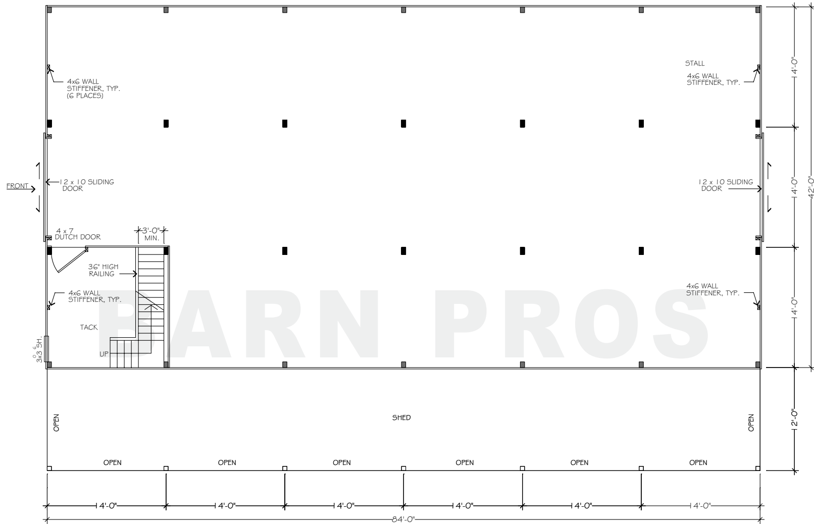
FLOORPLAN - LOWER
