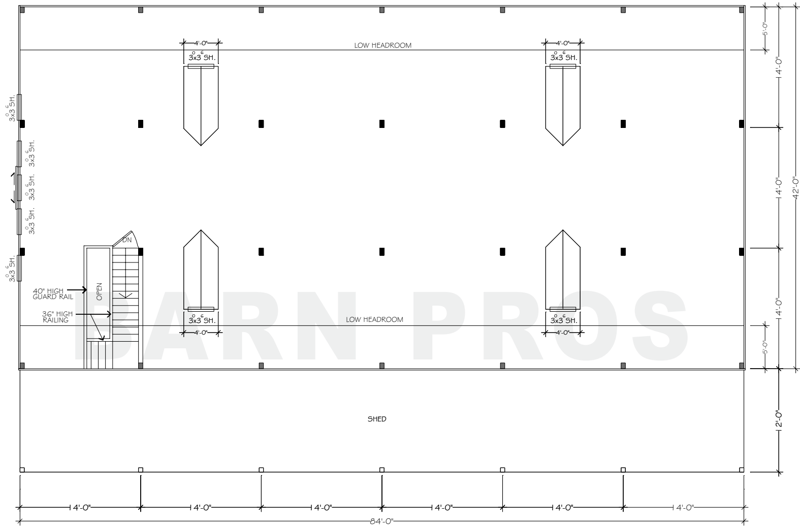
FLOORPLAN - UPPER
