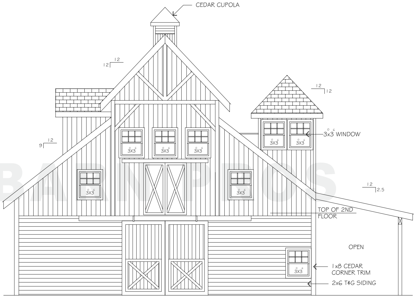
FRONT ELEVATION
