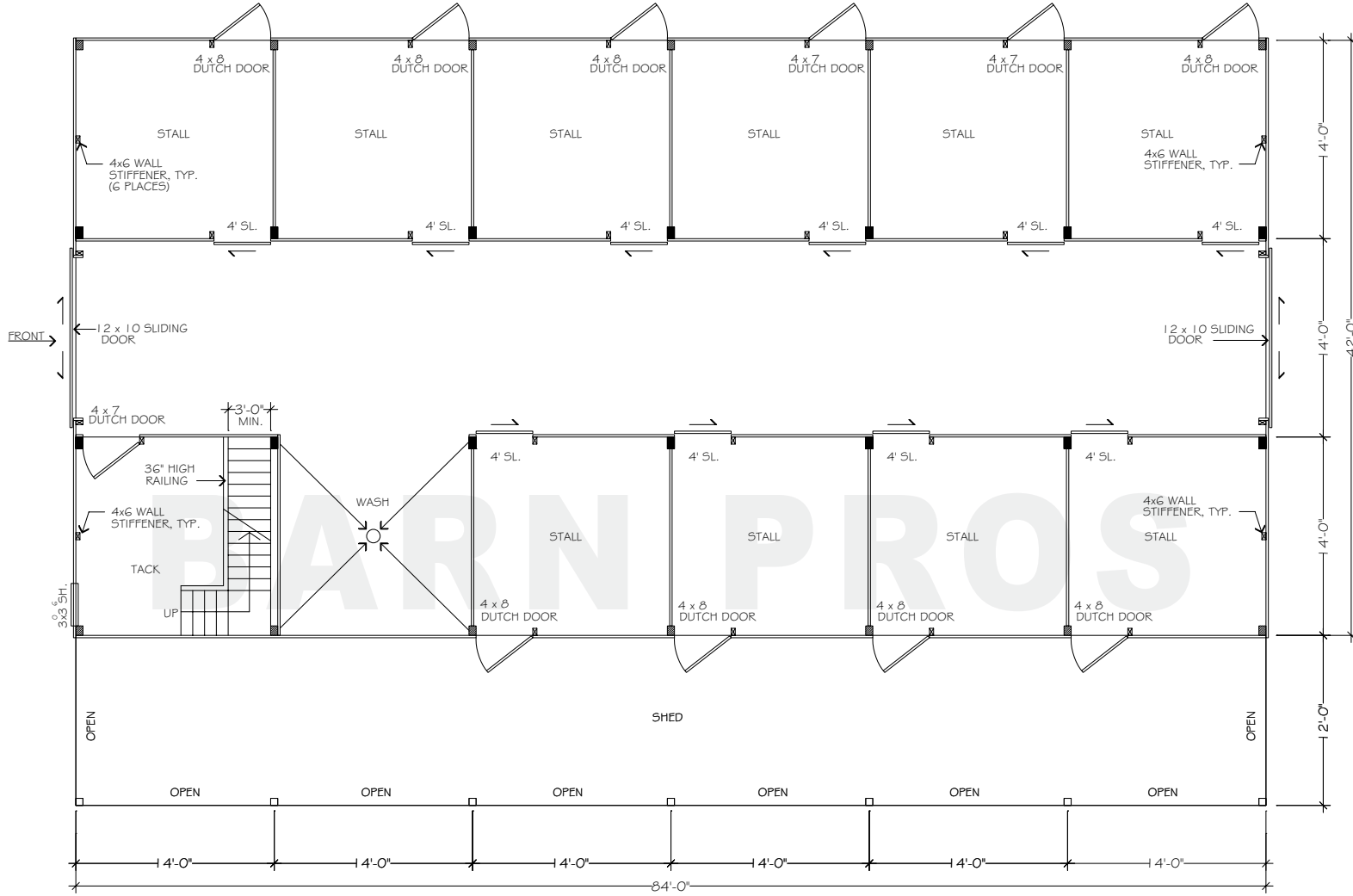
FLOORPLAN - LOWER
