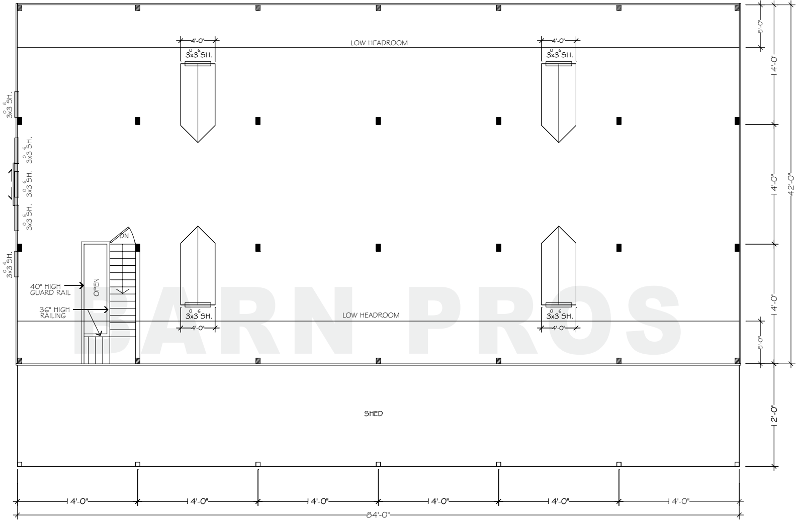
FLOORPLAN - UPPER
