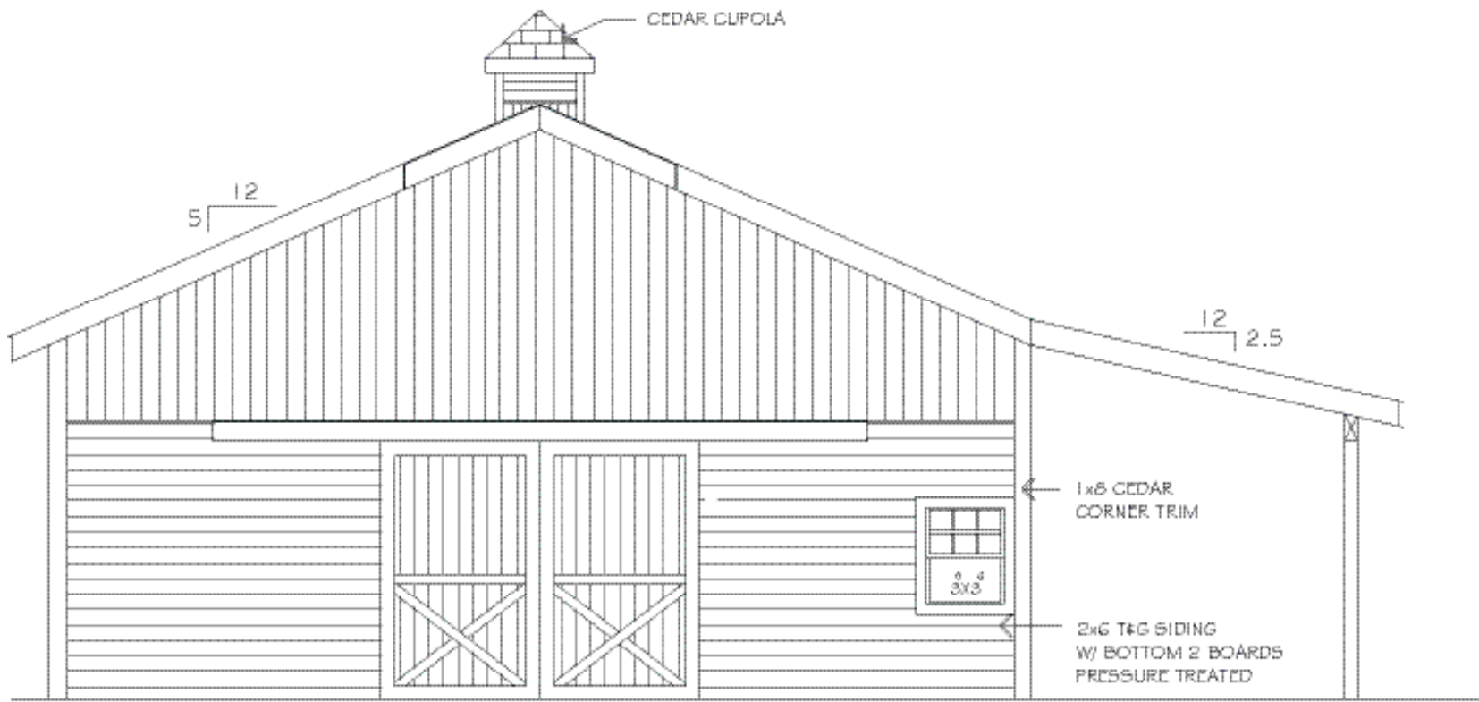
FRONT ELEVATION
