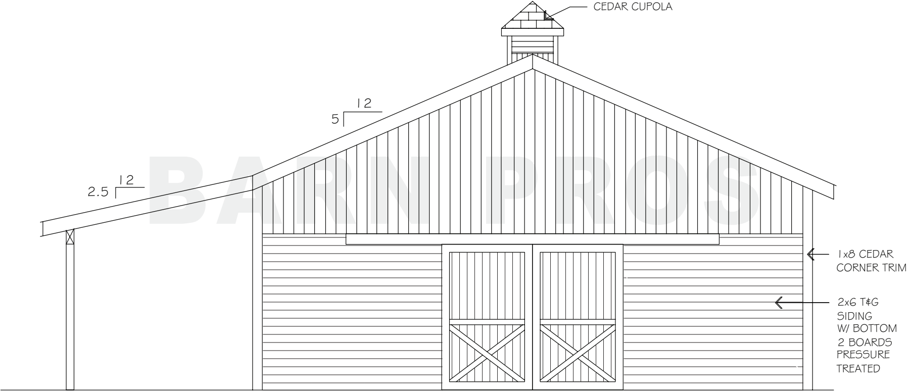
REAR ELEVATION
