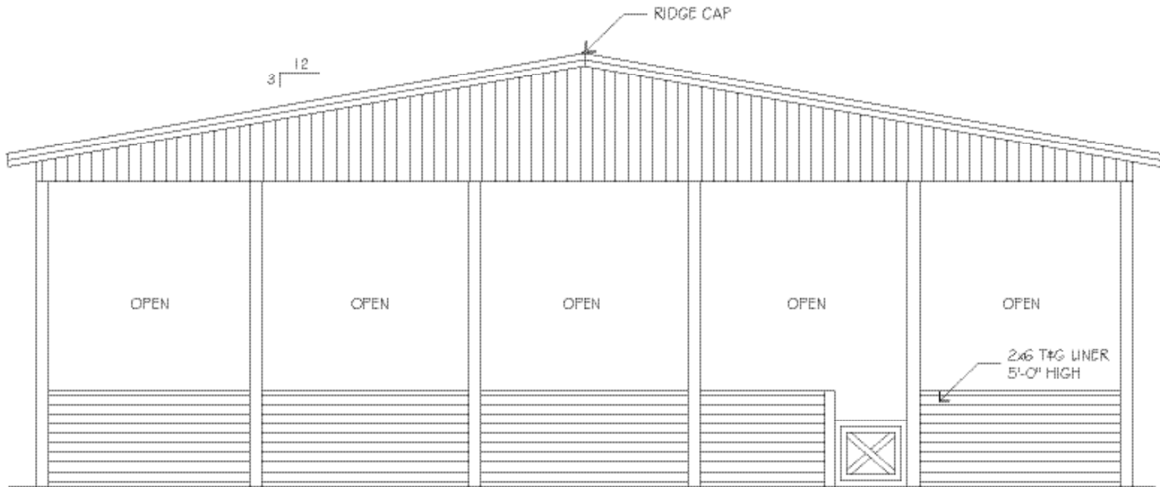
FRONT ELEVATION
