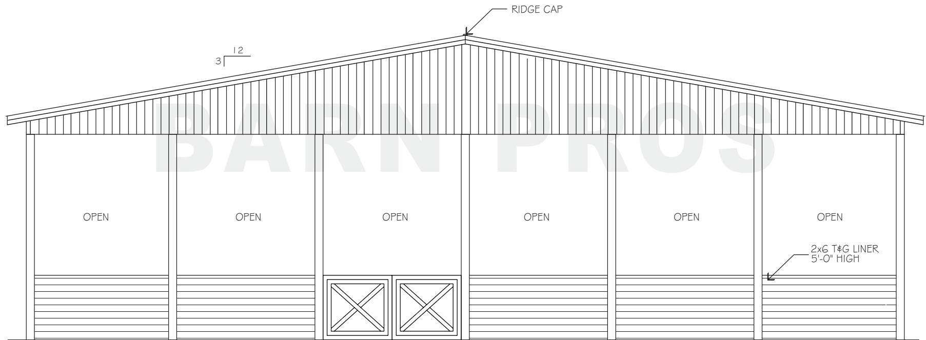
REAR ELEVATION
